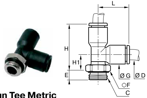
3193 Male Run Tee Metric Tube to Tube to Male BSP or M5
