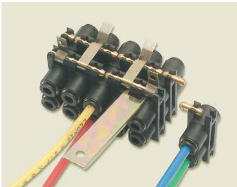
standard assembly
